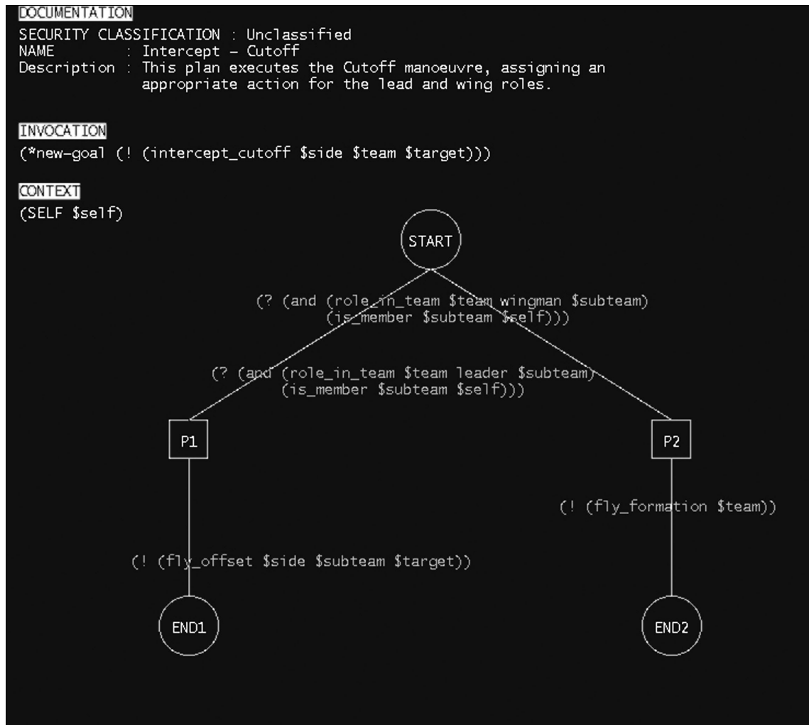
Figure 4. A dMARS Plan.
